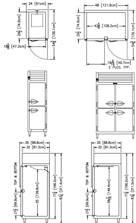
Section - R/ALT132DUT
