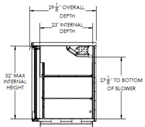
Elevation View
