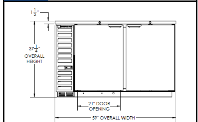
Elevation View
