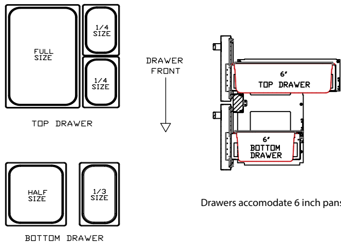
Pan Configuration
